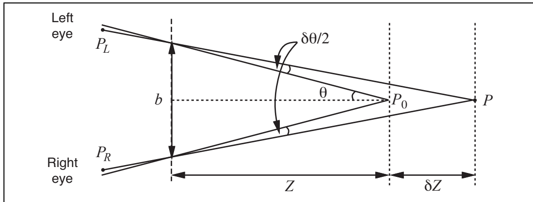
Figure 24.17 The relation between disparity and depth in stereopsis. The centers of projection of the two eyes are b apart, and the optical axes intersect at the fixation point P_0 . The point P in the scene projects to points P_L and P_R in the two eyes. In angular terms, the disparity between these is \delta\theta . See text.
