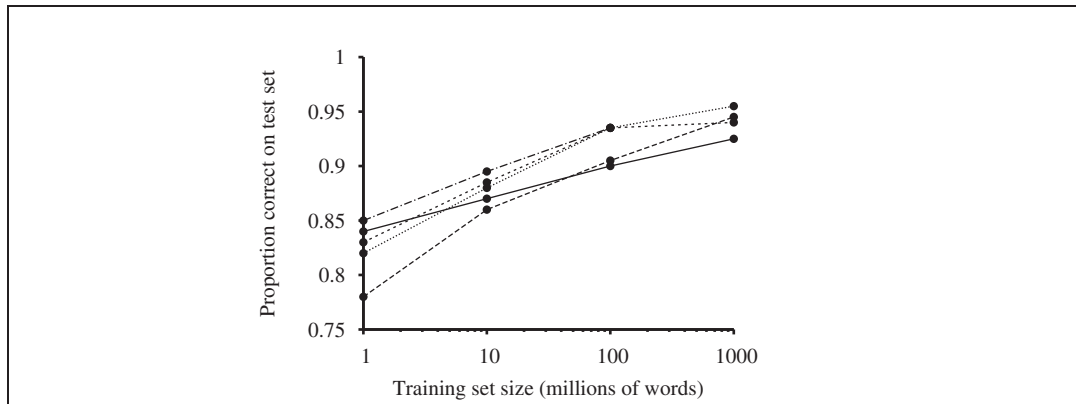
Figure 18.37 Learning curves for five learning algorithms on a common task. Note that there appears to be more room for improvement in the horizontal direction (more training data) than in the vertical direction (different machine learning algorithm). Adapted from Banko and Brill (2001).
