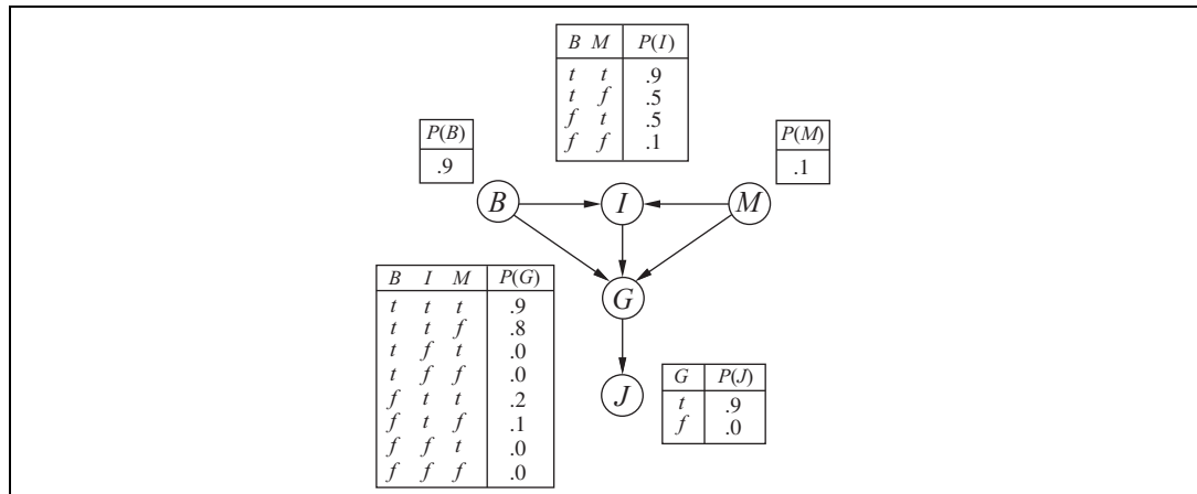
Figure 14.23 A simple Bayes net with Boolean variables B = BrokeElectionLaw , I = Indicted , M = PoliticallyMotivatedProsecutor , G = FoundGuilty , J = Jailed .
