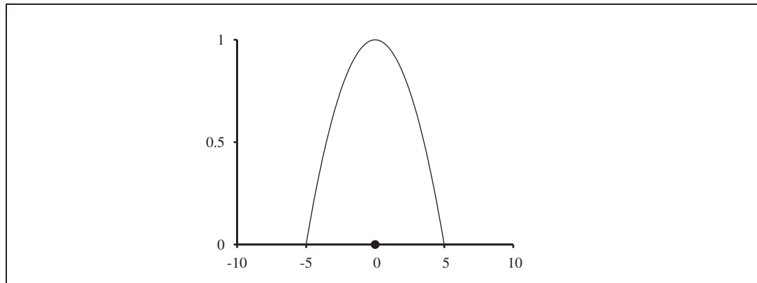
Figure 18.29 A quadratic kernel, \mathcal{K}(x) = \max(0, 1 - (2|x|/10)^2) , with kernel width = 10, centered on the query point x = 0 .
