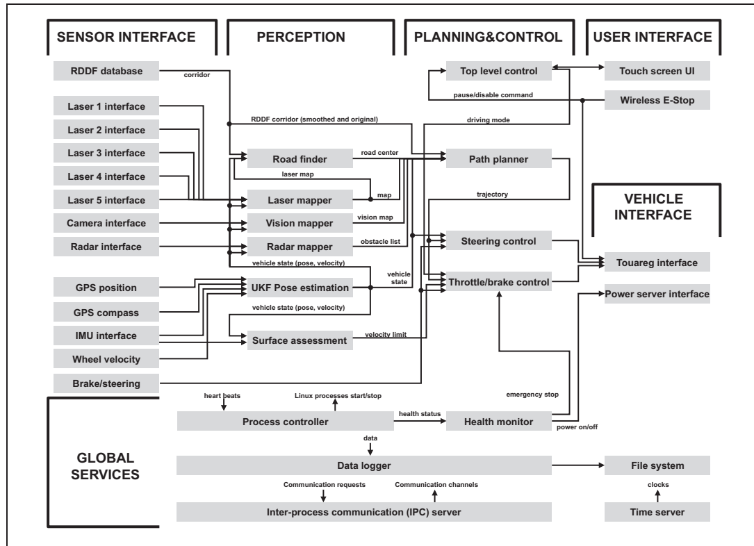
Figure 25.26 Software architecture of a robot car. This software implements a data pipeline, in which all modules process data simultaneously.
