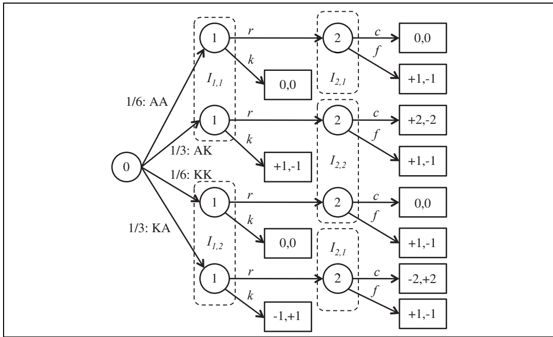
Figure 17.13 Extensive form of a simplified version of poker.
