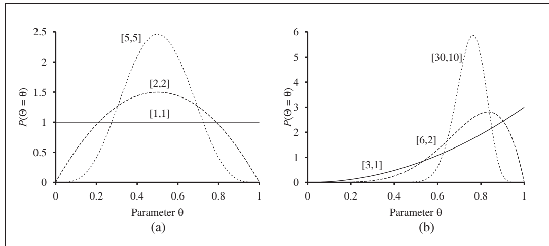
Figure 20.5 Examples of the beta [a, b] distribution for different values of [a, b] .
