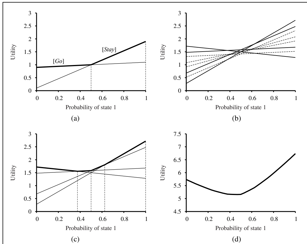
Figure 17.8 (a) Utility of two one-step plans as a function of the initial belief state b(1) for the two-state world, with the corresponding utility function shown in bold. (b) Utilities for 8 distinct two-step plans. (c) Utilities for four undominated two-step plans. (d) Utility function for optimal eight-step plans.
