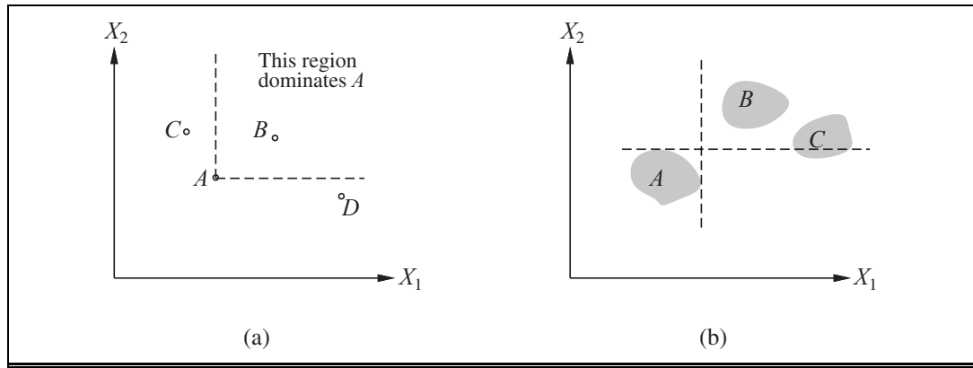
Figure 16.4 Strict dominance. (a) Deterministic: Option A is strictly dominated by B but not by C or D. (b) Uncertain: A is strictly dominated by B but not by C.
