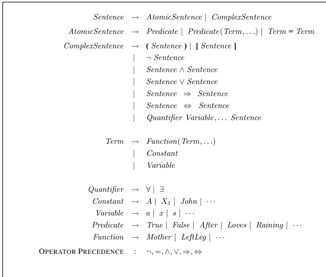
Figure 8.3 The syntax of first-order logic with equality, specified in Backus–Naur form (see page 1066 if you are not familiar with this notation). Operator precedences are specified, from highest to lowest. The precedence of quantifiers is such that a quantifier holds over everything to the right of it.
