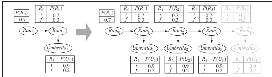
Figure 20.14 An unrolled dynamic Bayesian network that represents a hidden Markov model (repeat of Figure 15.16).
