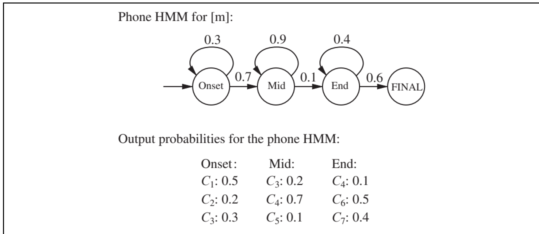
Figure 23.16 An HMM for the three-state phone [m]. Each state has several possible outputs, each with its own probability. The MFCC feature labels C_1 through C_7 are arbitrary, standing for some combination of feature values.
