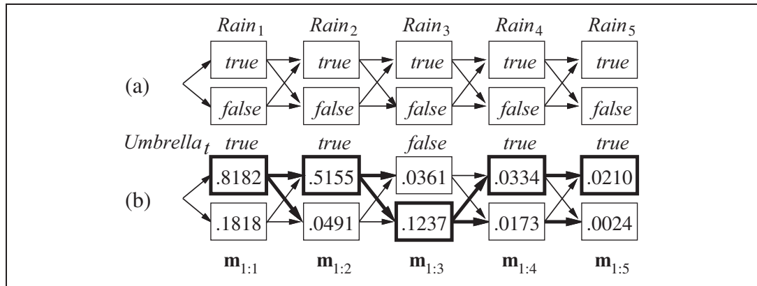
Figure 15.5 (a) Possible state sequences for Rain_t can be viewed as paths through a graph of the possible states at each time step. (States are shown as rectangles to avoid confusion with nodes in a Bayes net.) (b) Operation of the Viterbi algorithm for the umbrella observation sequence [true, true, false, true, true] . For each t , we have shown the values of the message m_{1:t} , which gives the probability of the best sequence reaching each state at time t . Also, for each state, the bold arrow leading into it indicates its best predecessor as measured by the product of the preceding sequence probability and the transition probability. Following the bold arrows back from the most likely state in m_{1:5} gives the most likely sequence.
