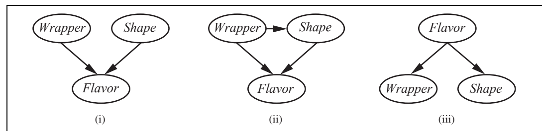
Figure 16.11 Three proposed Bayes nets for the Surprise Candy problem, Exercise 16.5.
