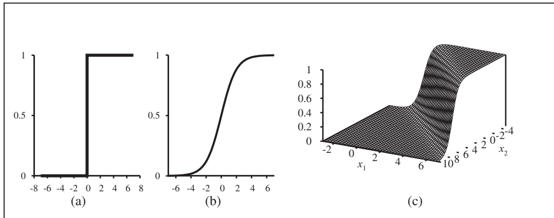
Figure 18.17 (a) The hard threshold function Threshold(\cdot) with 0/1 output. Note that the function is nondifferentiable at x = 0 . (b) The logistic function, Logistic(\cdot) = \frac{1}{1+e^{-z}} , also known as the sigmoid function. (c) Plot of a logistic regression hypothesis h_{\mathbf{w}}(\mathbf{x}) = Logistic(\mathbf{w} \cdot \mathbf{x}) for the data shown in Figure 18.15(b).
