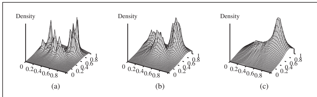
Figure 20.8 Density estimation using k -nearest-neighbors, applied to the data in Figure 20.7(b), for k=3, 10, and 40 respectively. k=3 is too spiky, 40 is too smooth, and 10 is just about right. The best value for k can be chosen by cross-validation.
