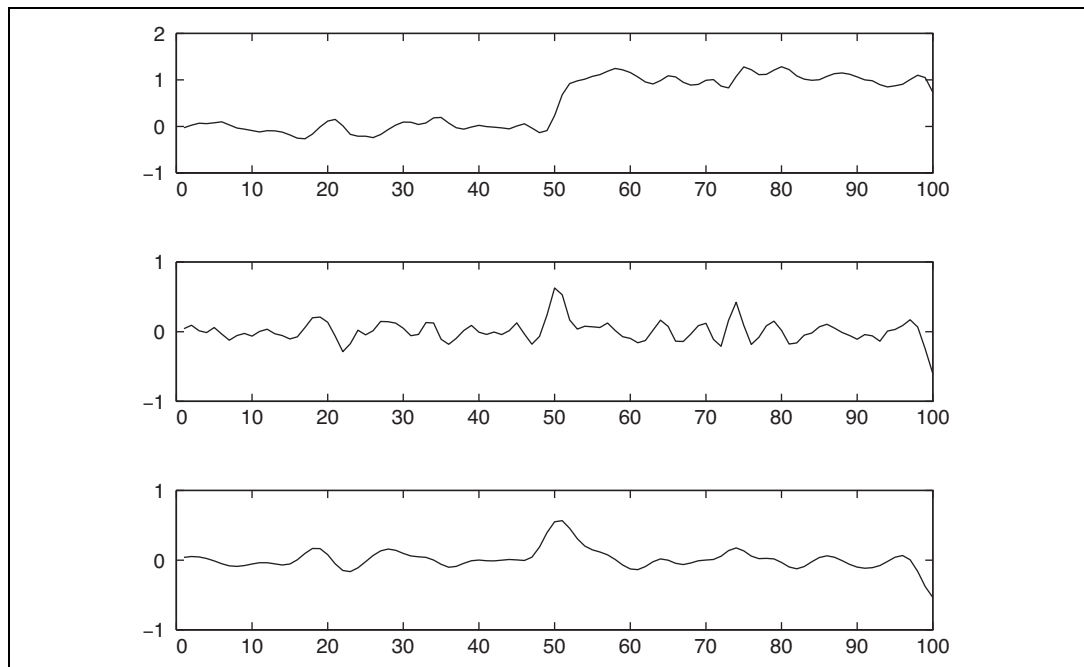
Figure 24.8 Top: Intensity profile I(x) along a one-dimensional section across an edge at x = 50 . Middle: The derivative of intensity, I'(x) . Large values of this function correspond to edges, but the function is noisy. Bottom: The derivative of a smoothed version of the intensity, (I * G_\sigma)' , which can be computed in one step as the convolution I * G'_\sigma . The noisy candidate edge at x = 75 has disappeared.
