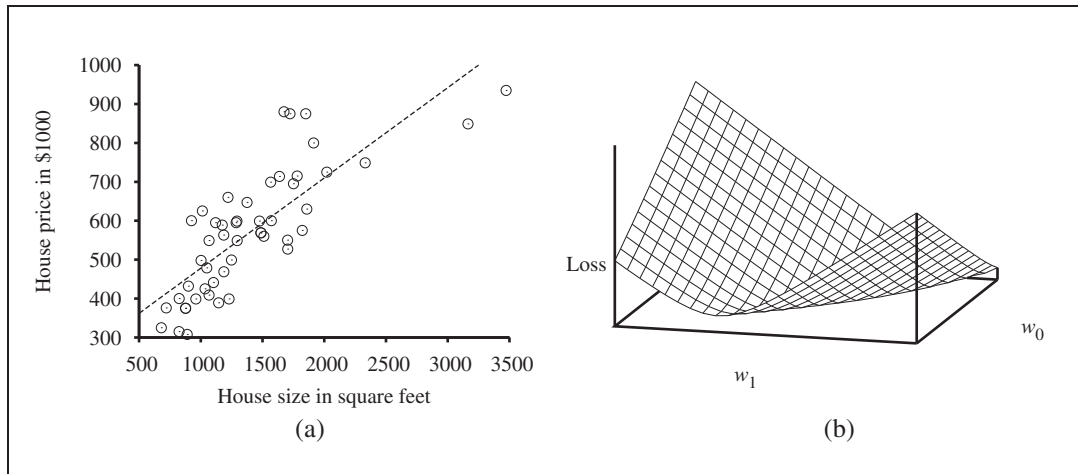
Figure 18.13 (a) Data points of price versus floor space of houses for sale in Berkeley, CA, in July 2009, along with the linear function hypothesis that minimizes squared error loss: \hat{y} = 0.232x + 246 . (b) Plot of the loss function \sum_j (y_j - (w_1 x_j + w_0))^2 for various values of w_0, w_1 . Note that the loss function is convex, with a single global minimum.
