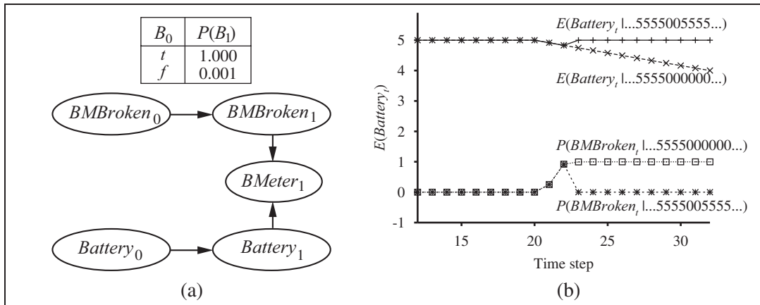
Figure 15.15 (a) A DBN fragment showing the sensor status variable required for modeling persistent failure of the battery sensor. (b) Upper curves: trajectories of the expected value of \text{Battery}_t for the “transient failure” and “permanent failure” observation sequences. Lower curves: probability trajectories for BMBroken given the two observation sequences.
