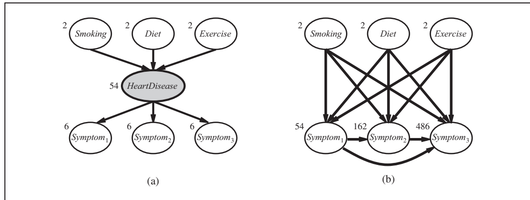
Figure 20.10 (a) A simple diagnostic network for heart disease, which is assumed to be a hidden variable. Each variable has three possible values and is labeled with the number of independent parameters in its conditional distribution; the total number is 78. (b) The equivalent network with HeartDisease removed. Note that the symptom variables are no longer conditionally independent given their parents. This network requires 708 parameters.
